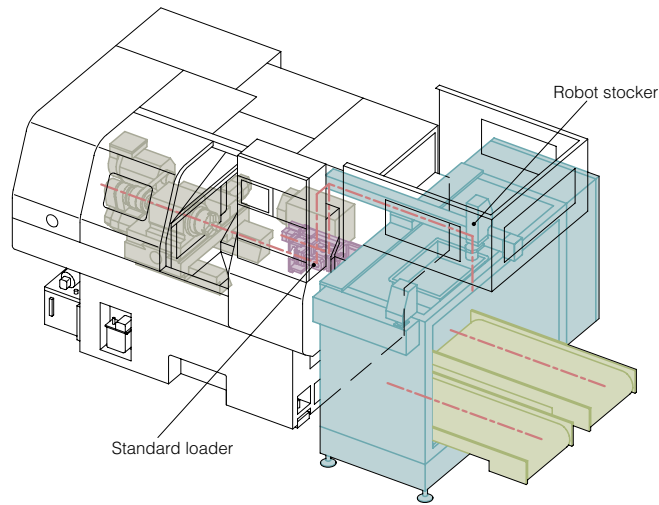
Robot stocker system (standard)
