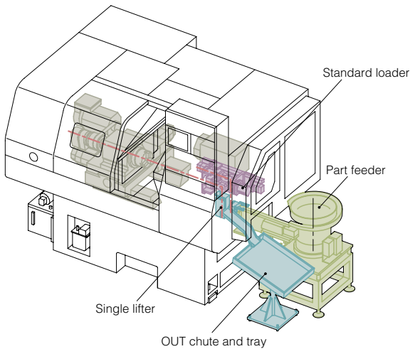
System with part feeder underneath (semi-standard)
