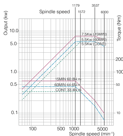
SP1 Torque diagram
